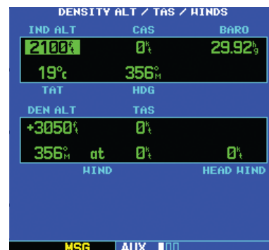
Figure 8-5 Density Alt/TAS/Winds Page
