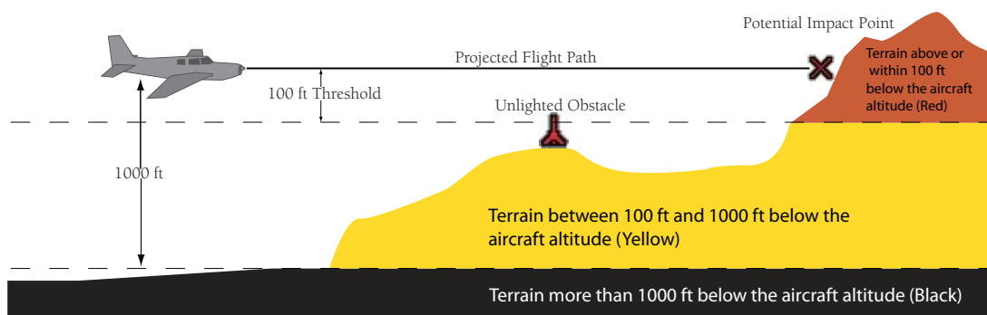
Figure 11-1 Terrain Altitude/Color Correlation for TAWS
