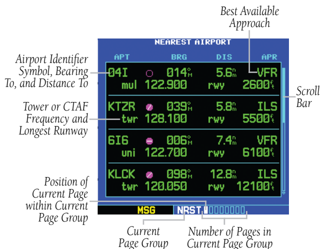
Figure 7-6 Nearest Airport Page
