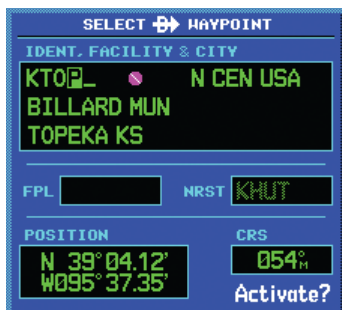
Figure 5-33 Select Waypoint Page
