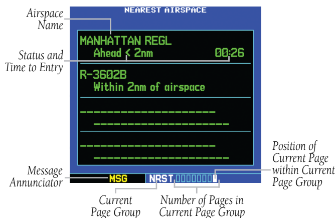
Figure 7-18 Nearest Airspace Page
