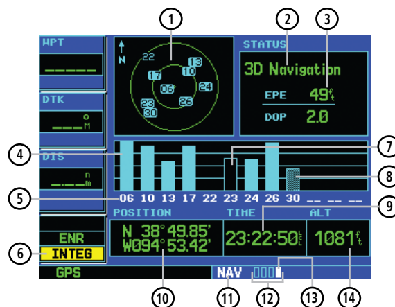
Figure 2-47 Satellite Status Page
