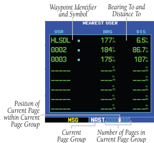
Figure 7-13 Nearest User Waypoint Page
